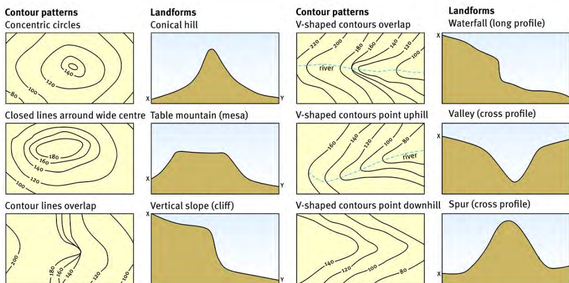
Figure 7 Contours and their landforms
